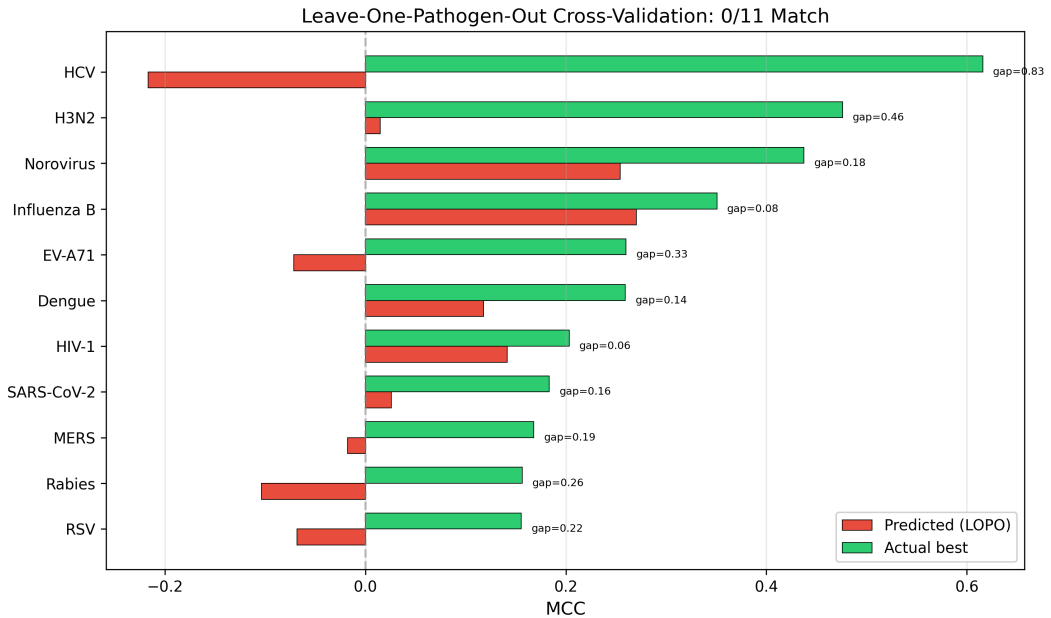
Figure 4.9: LOPO cross-validation results. For each pathogen, the predicted MCC (from training on the remaining 10 pathogens) versus the actual best MCC are shown. The 0/11 match rate is itself null-consistent under random-combination permutation ( P \approx 0.96 ); the figure should therefore be read as visualising the oracle-vs-generalised MCC gap (mean 0.265) rather than as standalone proof of non-generalisation.
