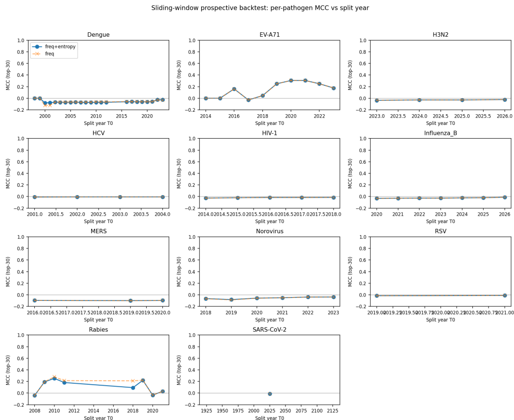
Figure 3.3: Per-pathogen MCC trajectory across split years for the sliding-window prospective backtest. The two pathogens above chance (EV-A71, Rabies) exhibit positive Top-30 MCC across multiple windows; Influenza B partially exceeds chance (AUROC 0.70) and the remaining eight cluster near zero (grand mean AUROC 0.539). Per-pathogen window counts and year ranges archived in sliding_window_prospective_backtest_summary.csv .
