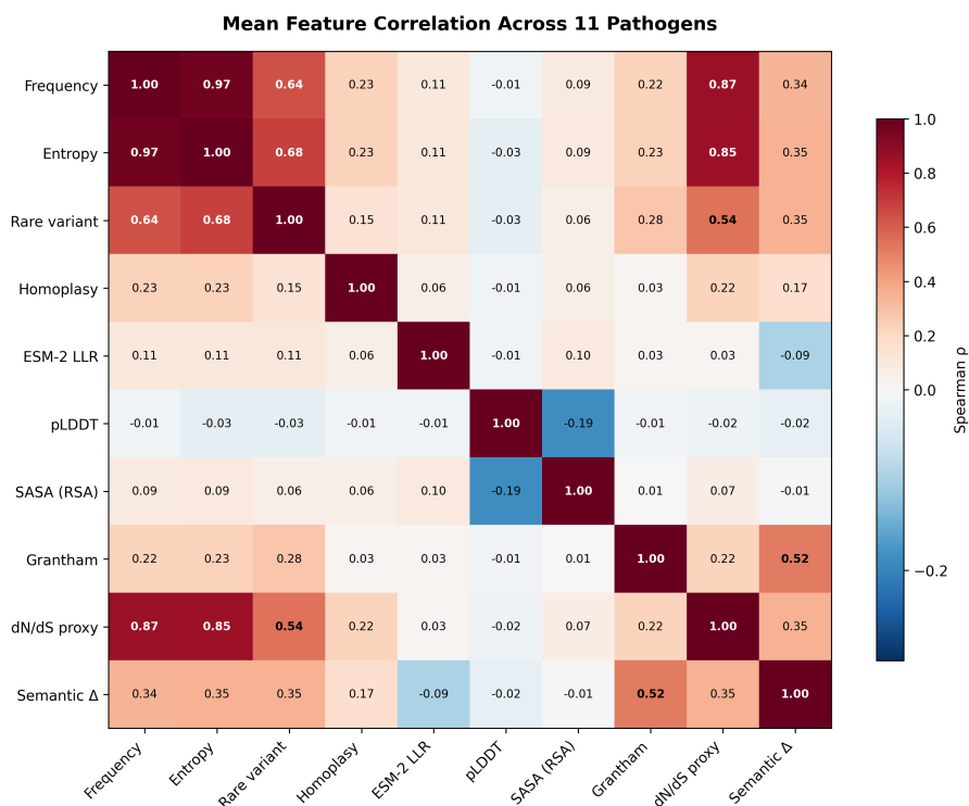
Figure 4.12: Mean pairwise Spearman correlation among 10 features across 11 pathogens. Three clusters are evident: frequency-derived features (freq, entropy, rare variant, dN/dS proxy) are highly correlated ( \rho > 0.54 ); deep learning features (ESM-2 masked-marginal score, semantic change) show weak negative correlation ( \rho = -0.09 ); and structure-based features (pLDDT, SASA) are weakly anti-correlated ( \rho = -0.19 ). Homoplasy is the most independent feature ( |\rho| \leq 0.233 with all others).
