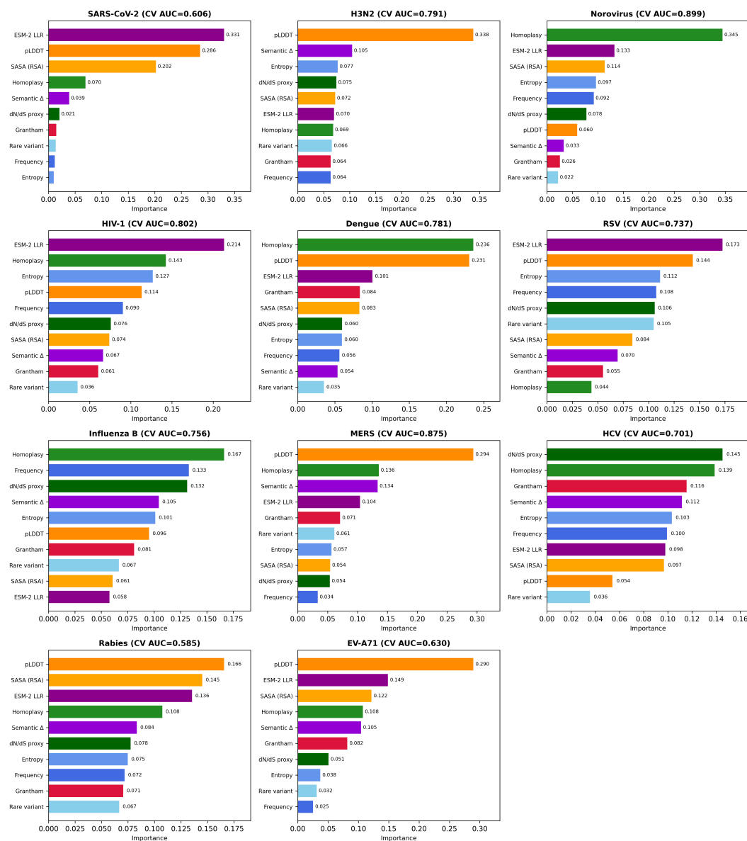
Figure 4.11: Random Forest feature importance for Layer A prediction across 11 pathogens (10 features). Bar colors indicate feature category: blue (frequency-based), green (phylogeny/evolutionary), purple (deep learning), orange (structure), crimson (chemical property). Cross-validation AUC is shown in each panel title. The dominant feature differs across pathogens: ESM-2 for SARS-CoV-2, pLDDT for H3N2 and Rabies, homoplasy for Norovirus and Dengue.
