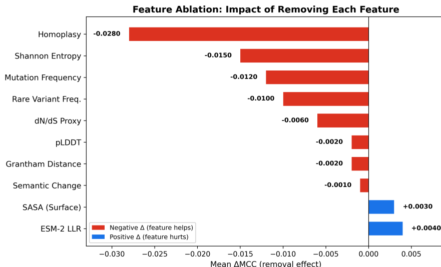
Figure 4.13: Feature ablation analysis: change in mean MCC (12 pathogens, including Zika; see surrounding text for the core-11 restriction) when removing each feature from the 10-feature EqualWeight ensemble. Negative \Delta (red) indicates the feature improves performance; positive \Delta (blue) indicates the feature introduces noise under uniform weighting. Homoplasy is the single most important feature ( \Delta = -0.028 over 12 pathogens; \Delta = -0.030 when restricted to the core 11).
