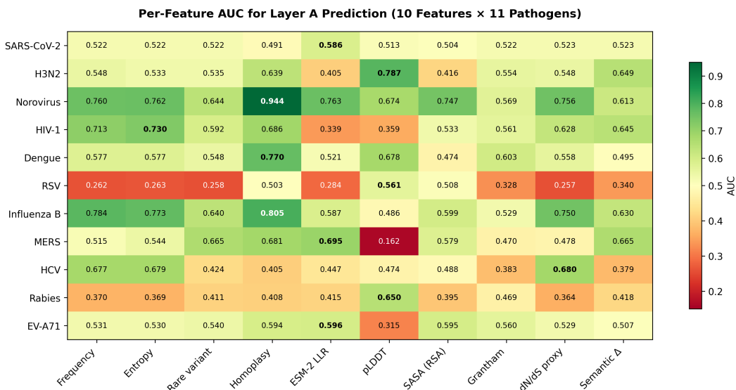
Figure 4.15: Per-feature AUC heatmap for Layer A prediction (11 pathogens, 10 features). Green indicates high discriminative power; red indicates inverse association ( AUC < 0.5 ). The best feature per pathogen is shown in bold. No single feature achieves the highest AUC for more than 3 of 11 pathogens.
