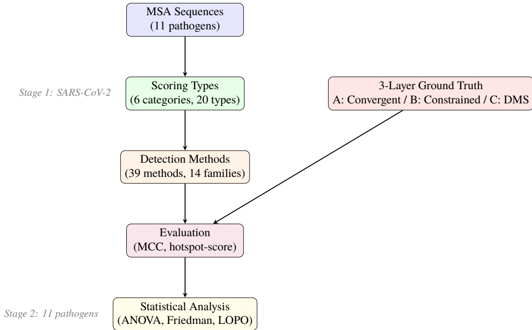
Figure 2.1: Overview of the MutBench experimental framework pipeline. Input multiple sequence alignment (MSA) data are processed through scoring types and detection methods, evaluated against a 3-layer ground truth, and analyzed using multiple statistical tests.
