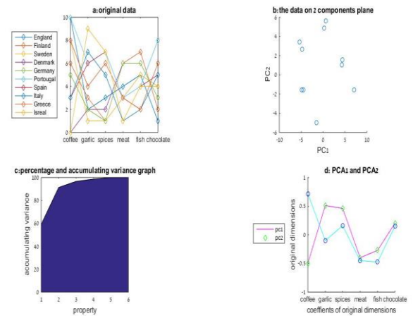
Figure 1: a- food consumption of different countries, b- PCA and plot of data in 2-dimension, c- percentage and accumulating variance graph, d- values of PC1 versus PC2
