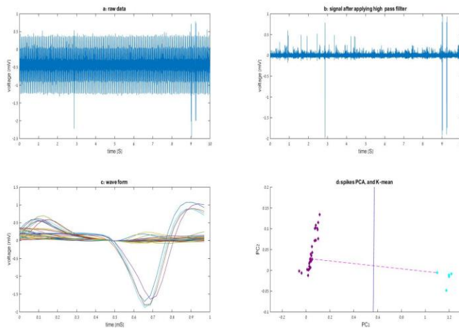
Figure 2: a- original data, b- b. afret filtering the noise (frequency below 300), c- wave form, d- spikes wave form and K-means clustering, separation line(blue) is perpendicular bisector to the line between to closet points (pink)
