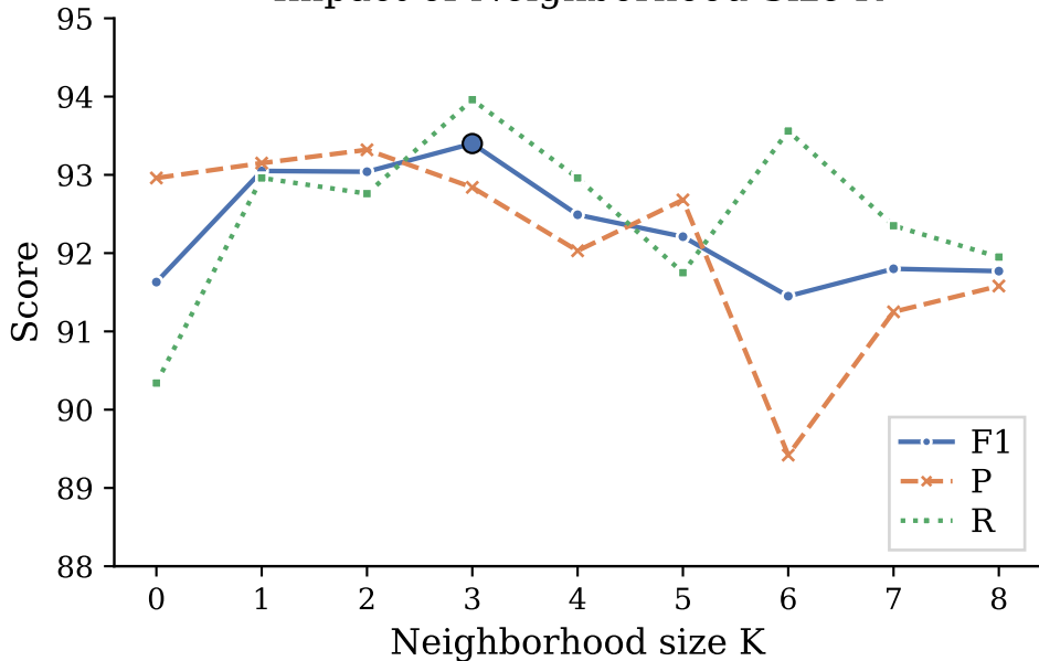
Impact of Neighborhood Size K
