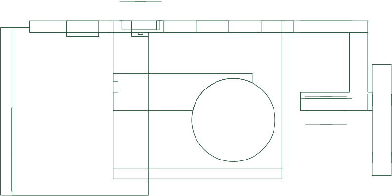
Overall: 84.20 x 41.70 mm
