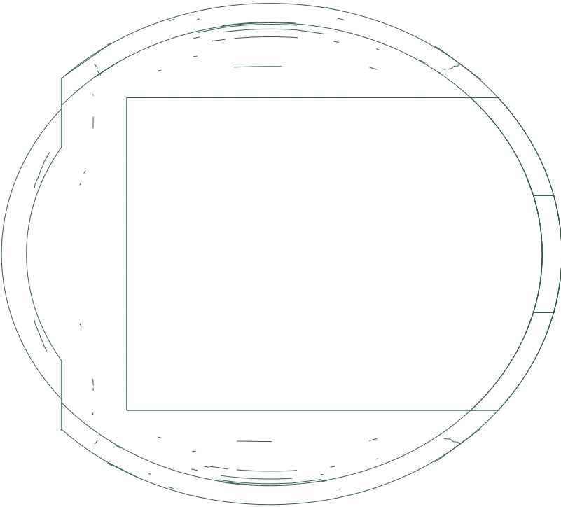
Overall: 86.04 x 77.20 mm
