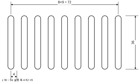
VENT DETAIL (C1/C3/C4/C6) 1:1.25
