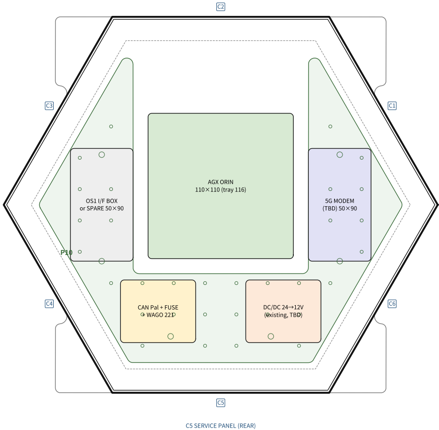
INTERNAL LAYOUT — TOP (cover removed) 1:3
