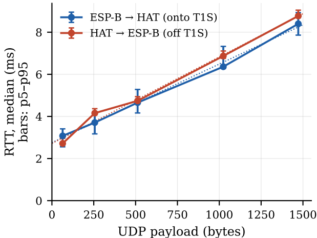
Fig. 2 RTT vs payload, linear fit (dotted)
