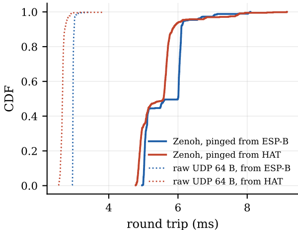
Fig. 8 Zenoh ping/pong vs raw UDP echo
