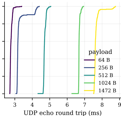
Fig. 1 Round-trip time across converter + 10BASE-T1S, by payload size measured on ESP-B (W5500) measured on the HAT node (LAN8651)
