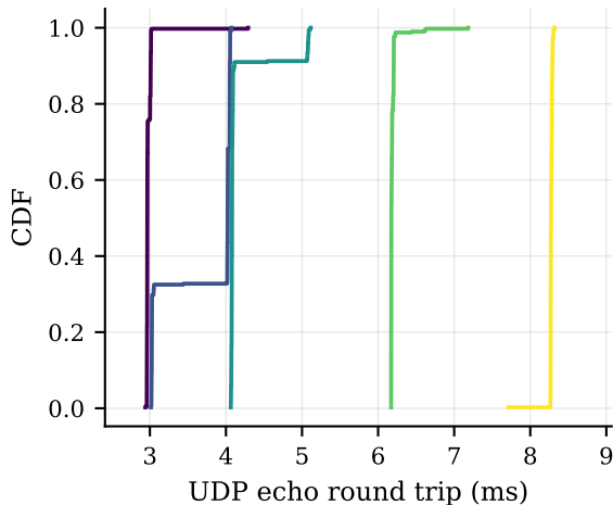
Fig. 1 Round-trip time across converter + 10BASE-T1S, by payload size measured on ESP-B (W5500) measured on the HAT node (LAN8651)
