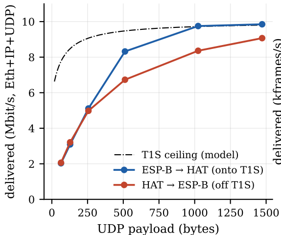
(a) throughput
