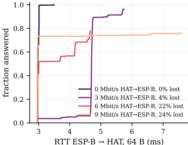
Fig. 6 Latency under reverse load
