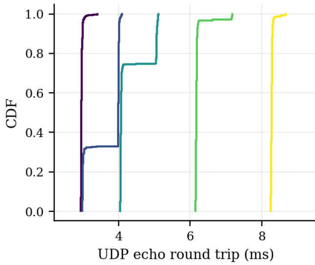
Fig. 1 Round-trip time across converter + 10BASE-T1S, by payload size measured on ESP-B (W5500)
