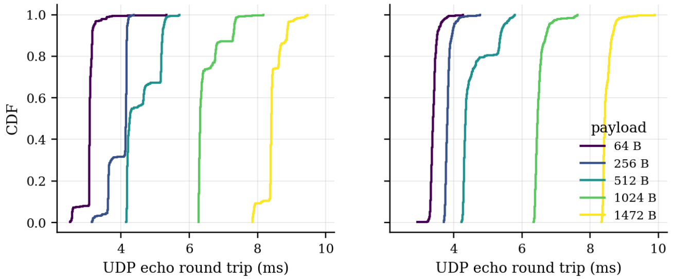
Fig. 1 Round-trip time across converter + 10BASE-T1S, by payload size measured on ESP-B (W5500) measured on the HAT node (LAN8651)
