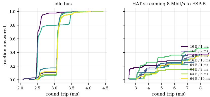
Fig. C3 CAN-like periodic messages, round trip from ESP-B; loaded: only probes sent while the load ran (curves end below 1 where probes were lost)
