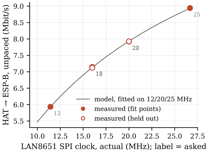
Fig. C2 SPI clock model, out-of-sample check
