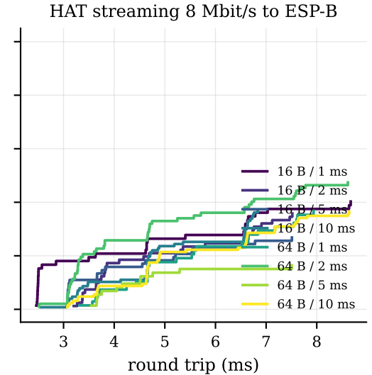
Fig. C3 CAN-like periodic messages, round trip from ESP-B; loaded: only probes sent while the load ran (curves end below 1 where probes were lost)
