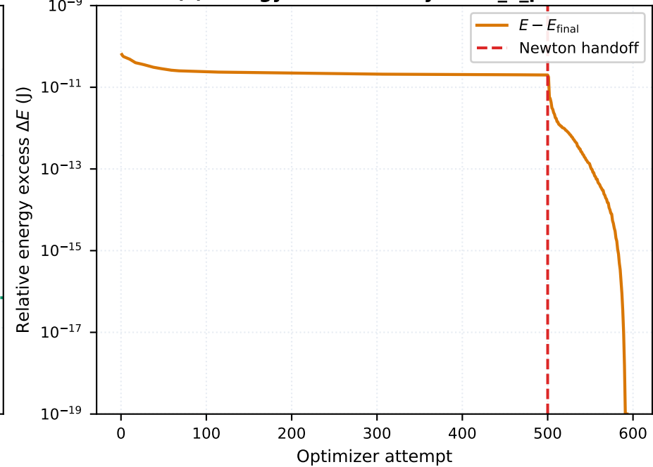
(c) Energy relaxation: cylinder_x_plus
