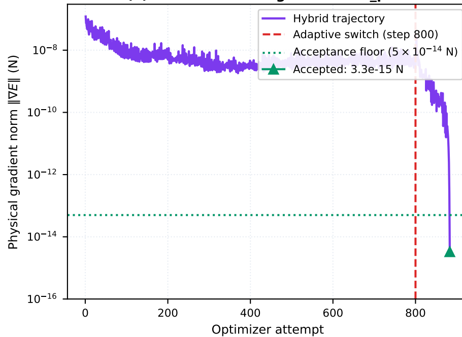
(e) Gradient convergence: twist_plus
