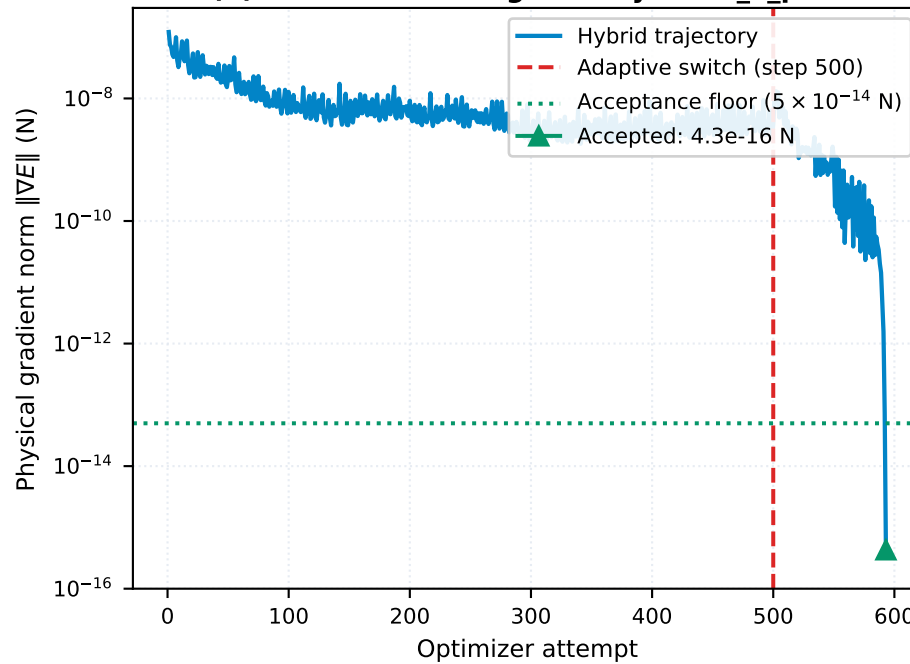
(b) Gradient convergence: cylinder_x_plus
