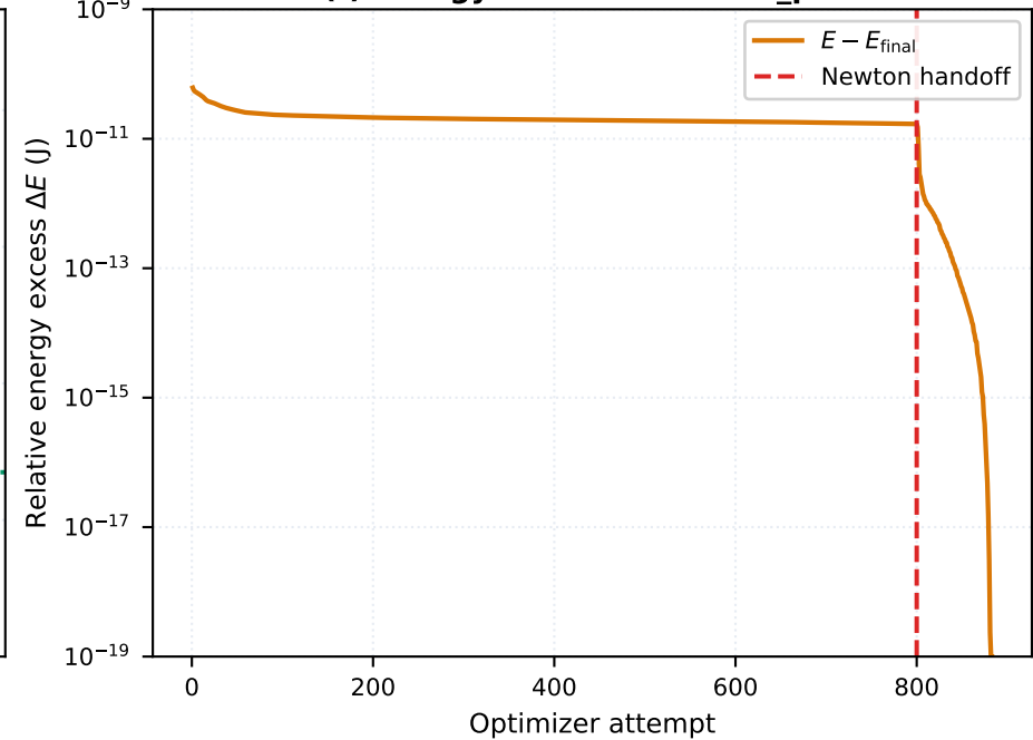
(f) Energy relaxation: twist_plus
