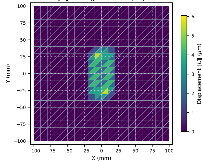
\|U\| Field (peak: 6.06 \mu\text{m} )
