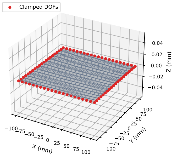
Initial: Clamped Plate (Fixed Edges)
