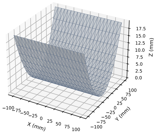
Initial: Clamped Plate (Fixed Edges)
