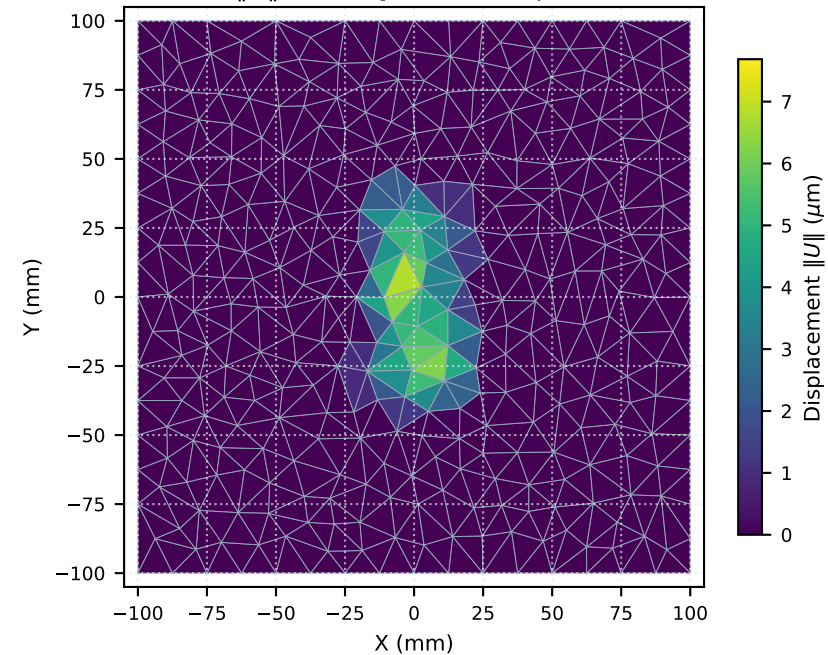
\|U\| Field (peak: 7.69 \mu\text{m} )
