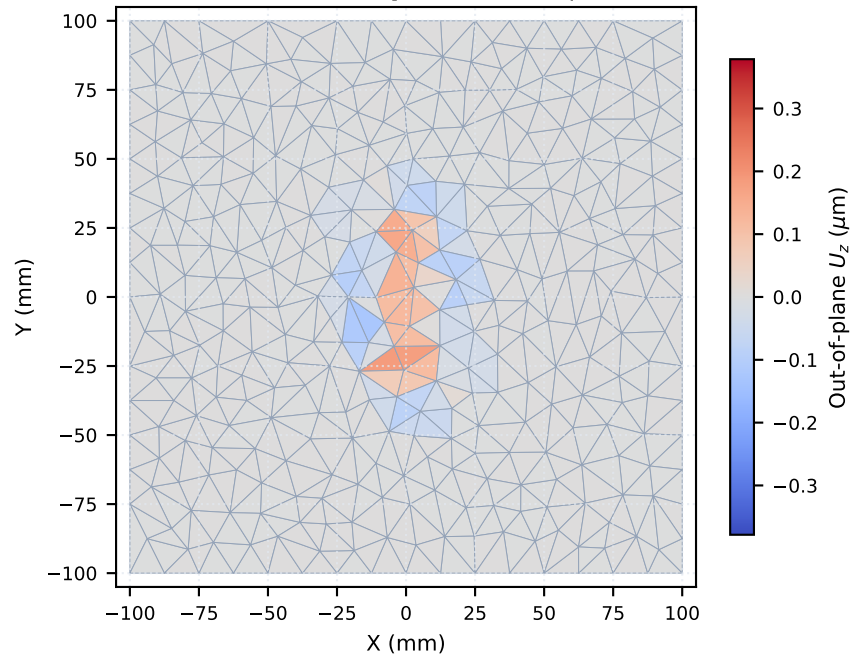
Deflection U_z (peak: +0.38 \mu\text{m} )
