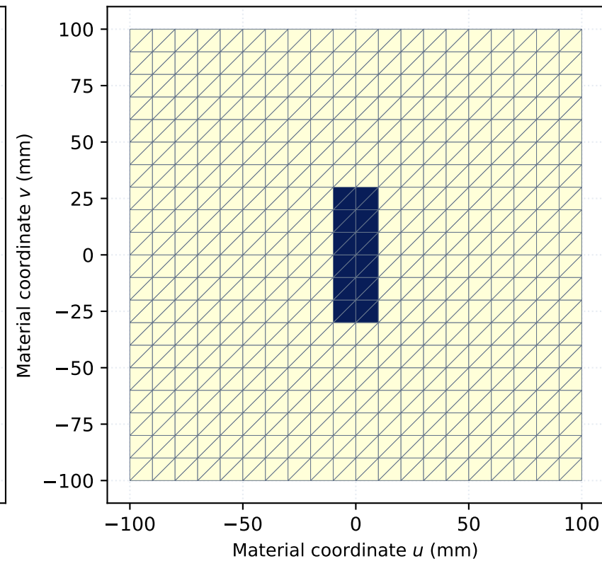
(b) Discrete mesh hit footprint (800 faces)
