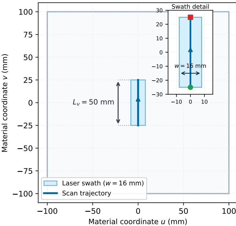
(a) Toolpath geometry on plate ( 0.2 \times 0.2 m)
