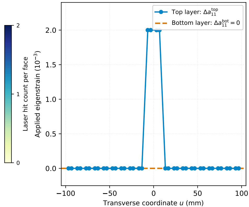
(c) Eigenstrain profile at centerline ( v = 0 )
