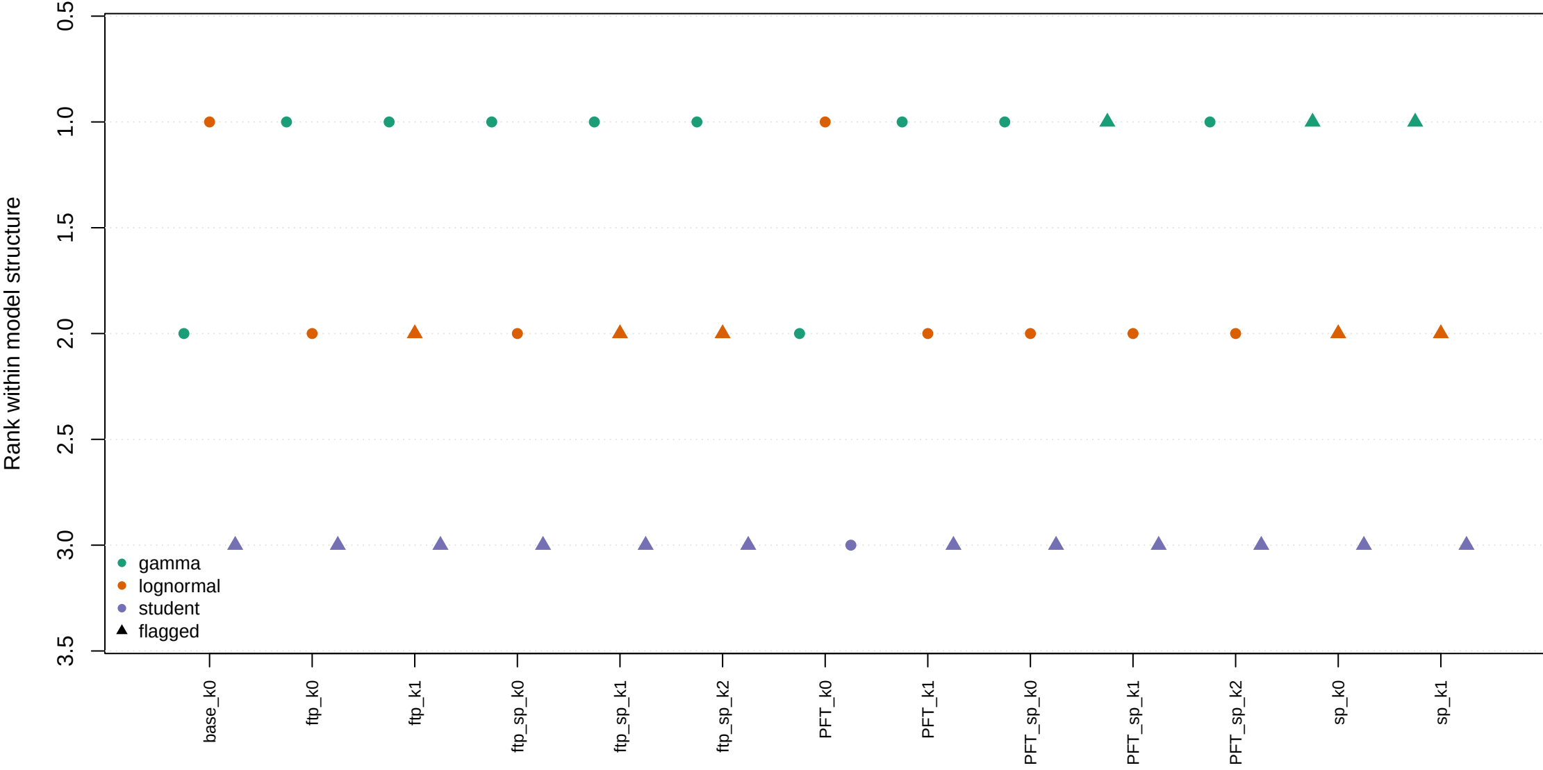
LOO distribution rank by model structure
