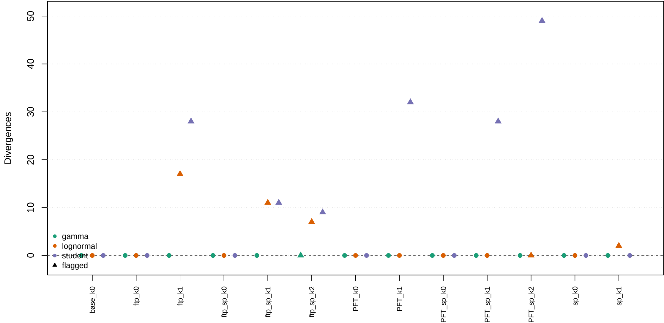
MCMC divergences by model structure and distribution
