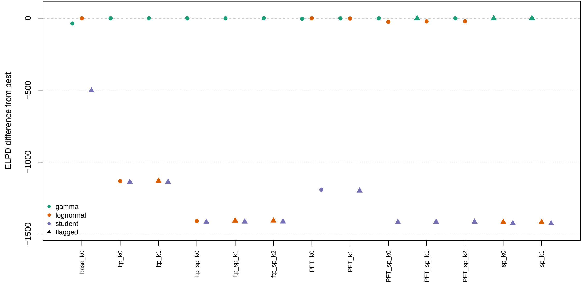
LOO distribution comparison by model structure
