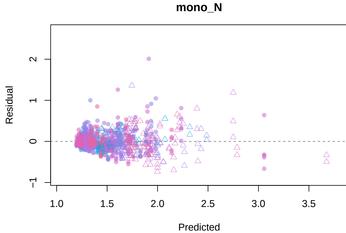
Residual vs Predicted by h1/h2: ftp_sp_k2_gamma
