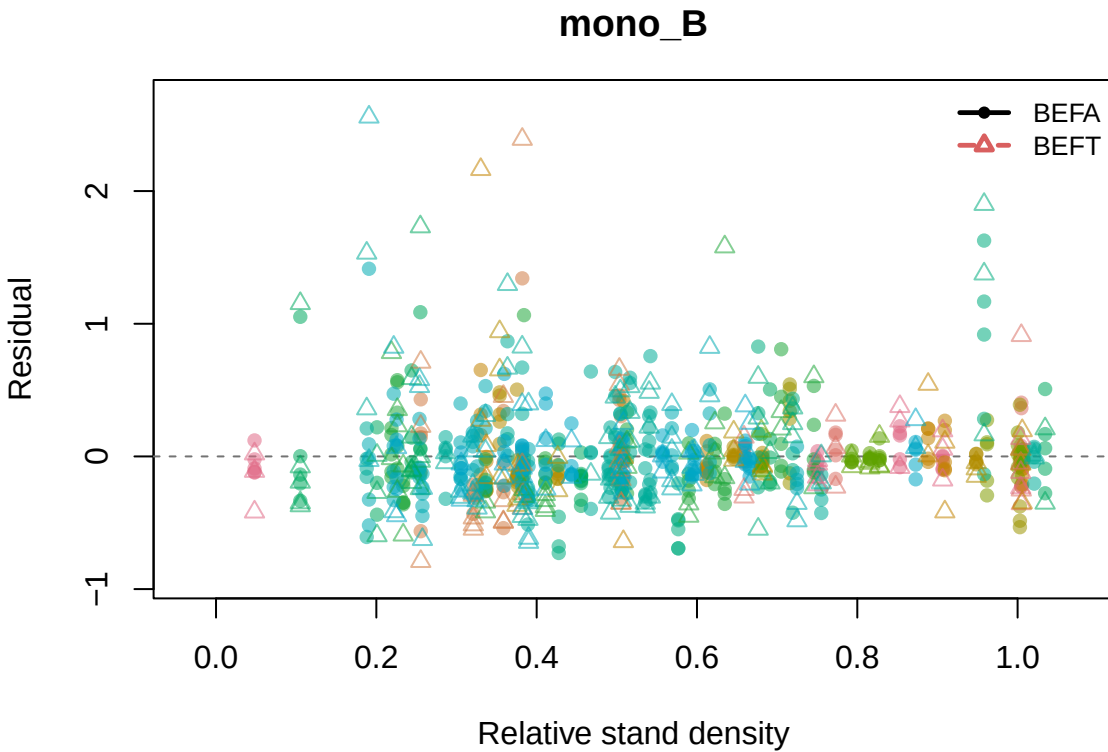
Residual vs Relative stand density by h1/h2: ftp_sp_k2_gamma
