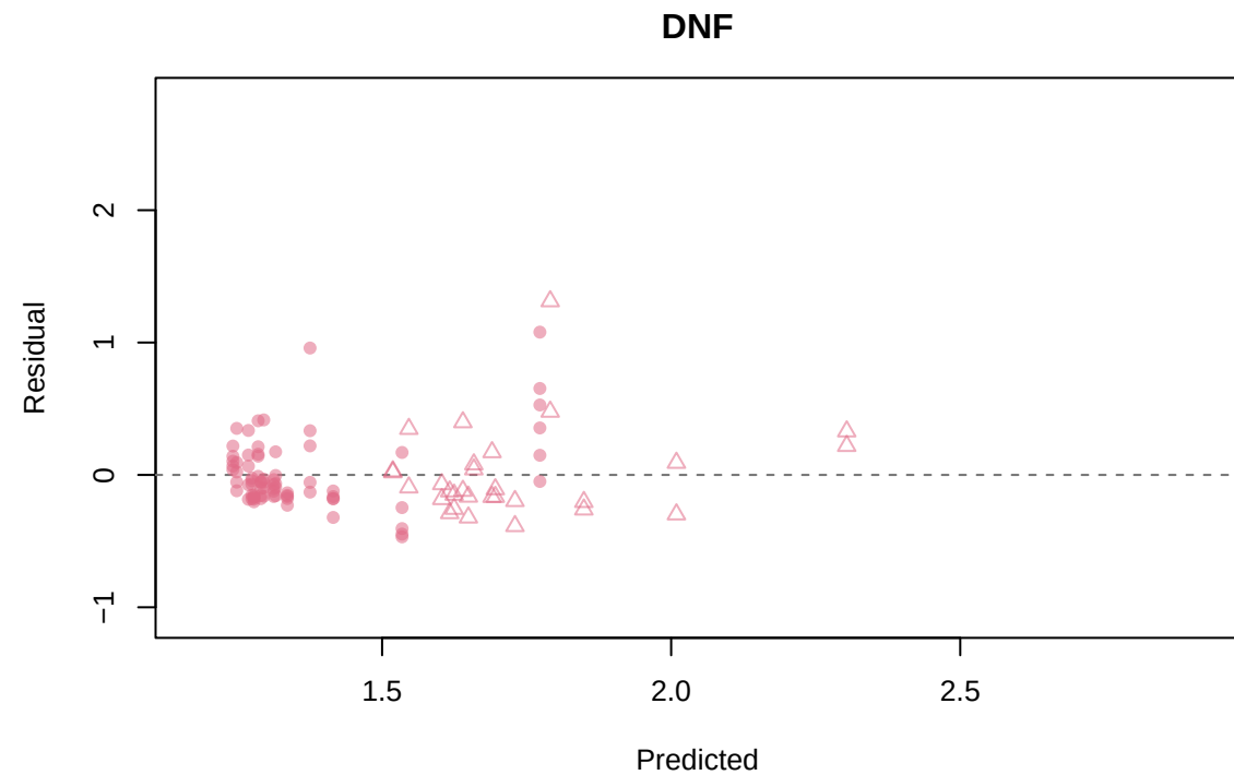
Residual vs Predicted by h1/h2: PFT_k0_gamma
