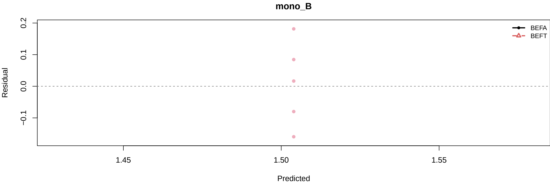
Residual vs Predicted by h1/h2: ftp_sp_k0_gamma
