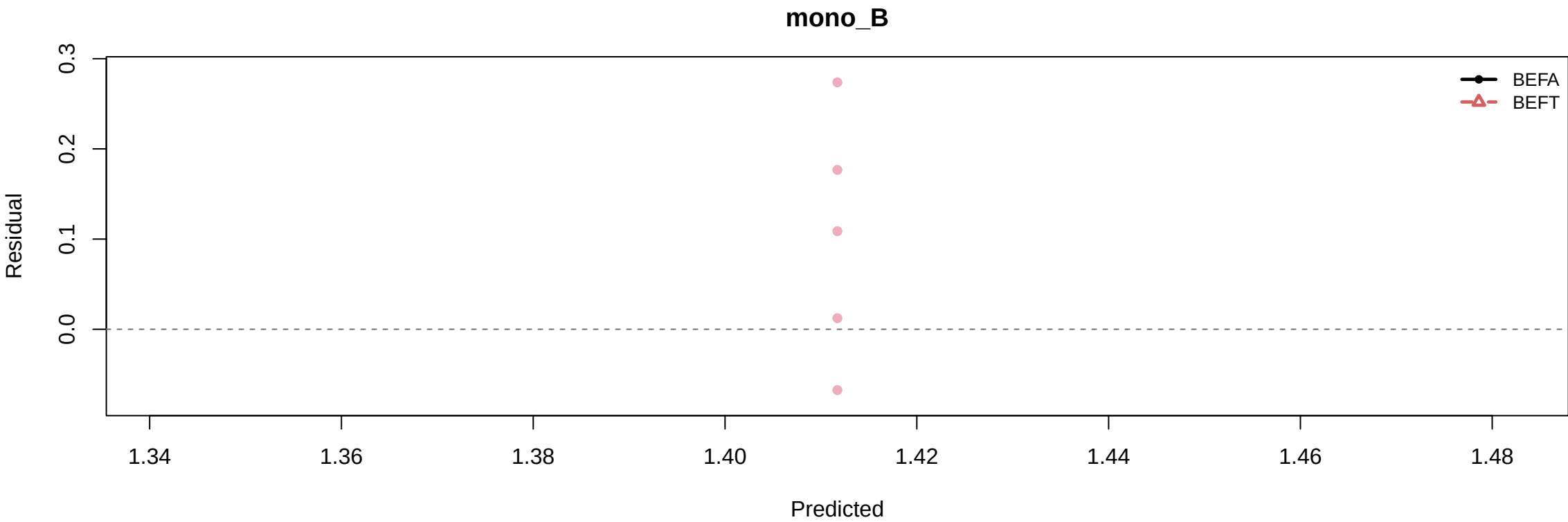
Residual vs Predicted by h1/h2: ftp_k0_gamma
