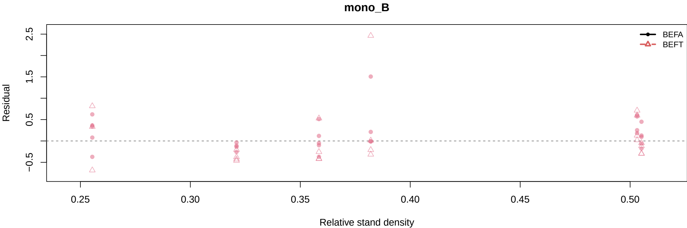
Residual vs Relative stand density by h1/h2: ftp_k1_gamma
