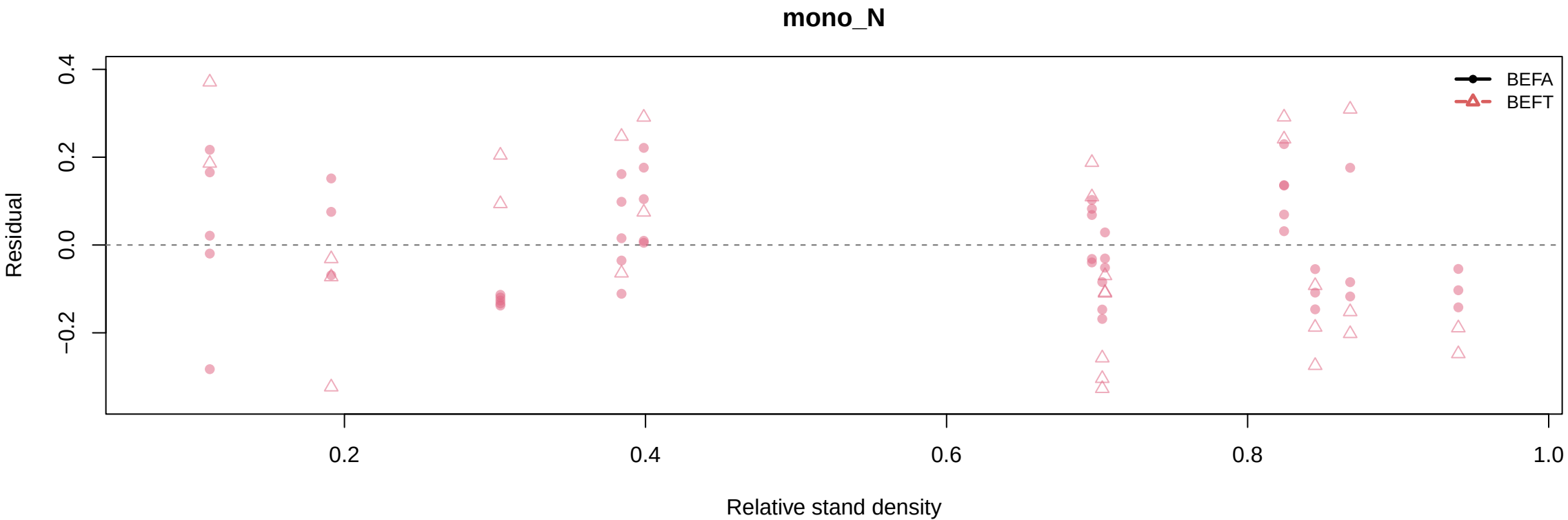
Residual vs Relative stand density by h1/h2: ftp_sp_k0_gamma
