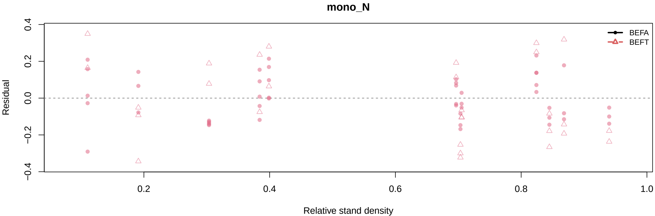
Residual vs Relative stand density by h1/h2: ftp_sp_k2_gamma
