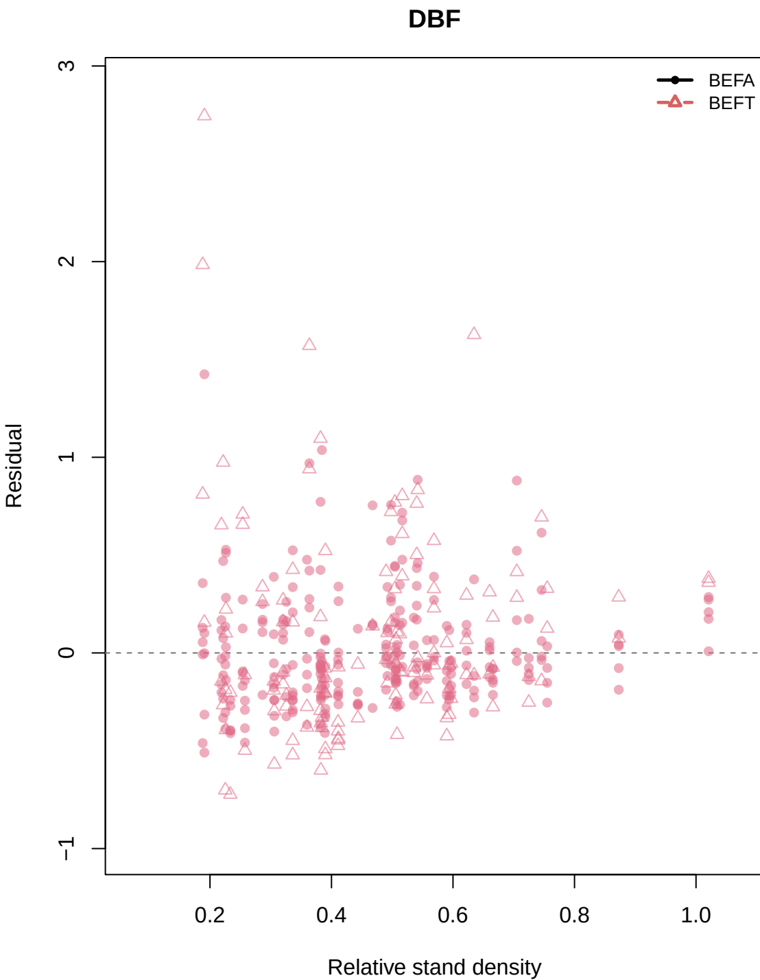
Residual vs Relative stand density by h1/h2: PFT_k1_gamma
