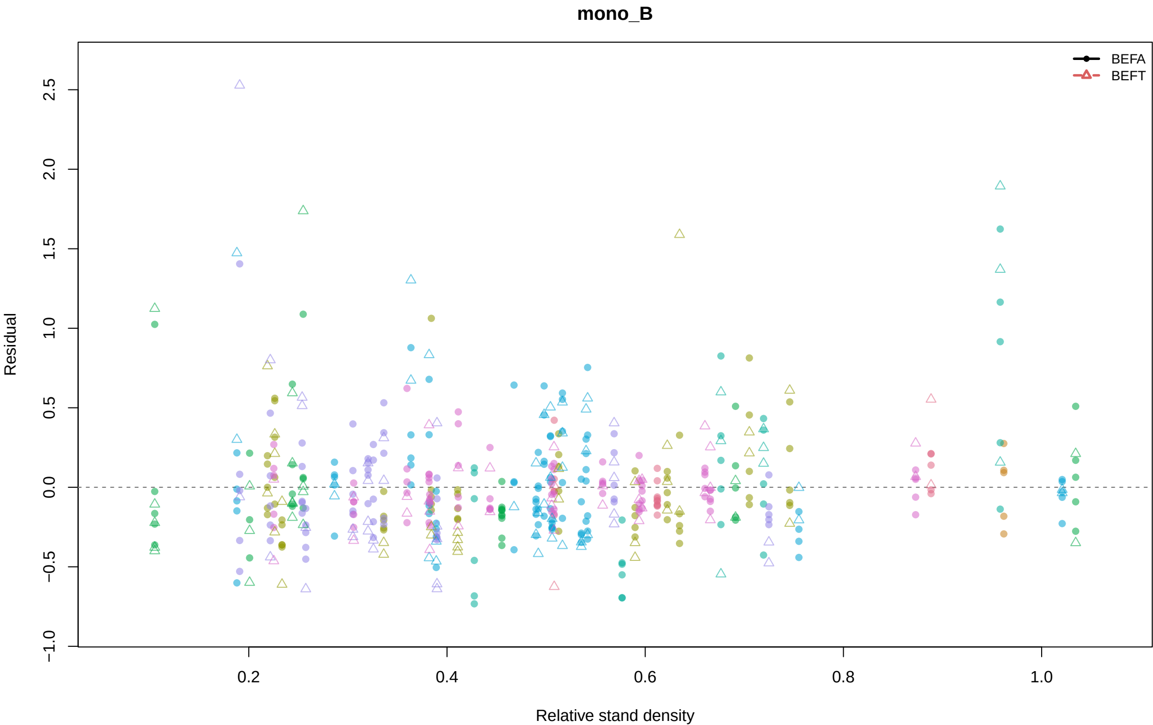
Residual vs Relative stand density by h1/h2: ftp_sp_k1_gamma
