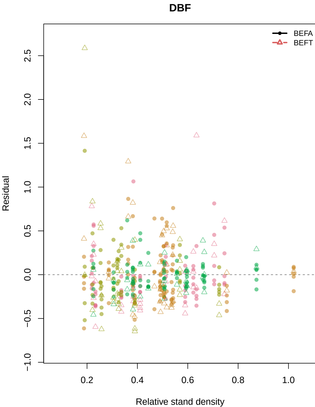
Residual vs Relative stand density by h1/h2: PFT_sp_k2_gamma
