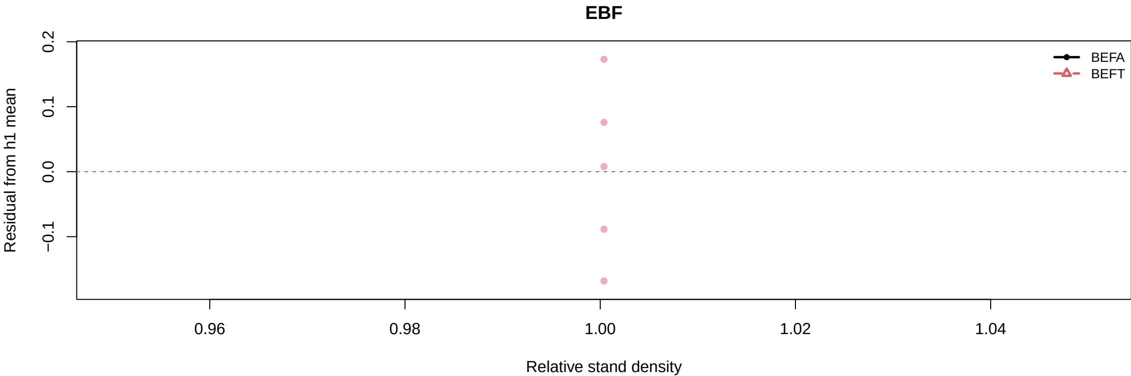
Residual from h1 mean vs rsd by h1/h2: PFT_sp_k0_gamma
