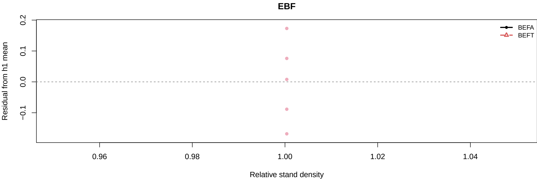
Residual from h1 mean vs rsd by h1/h2: PFT_sp_k1_gamma
