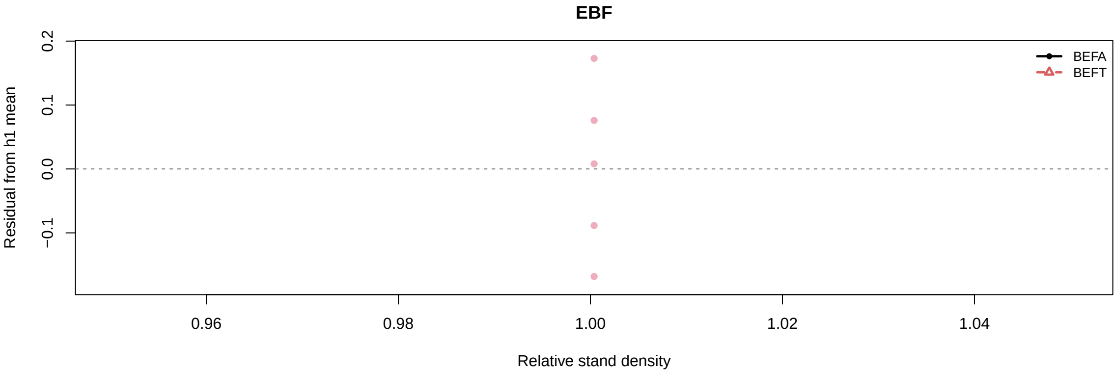
Residual from h1 mean vs rsd by h1/h2: PFT_k0_gamma
