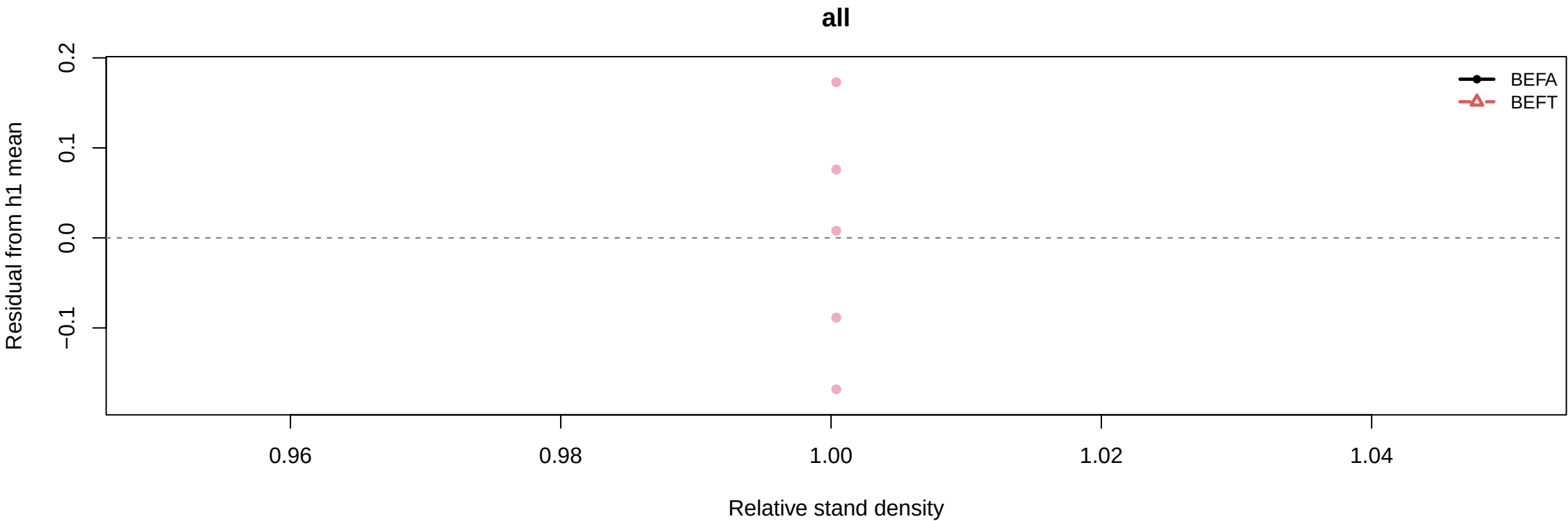
Residual from h1 mean vs rsd by h1/h2: base_k0_gamma
