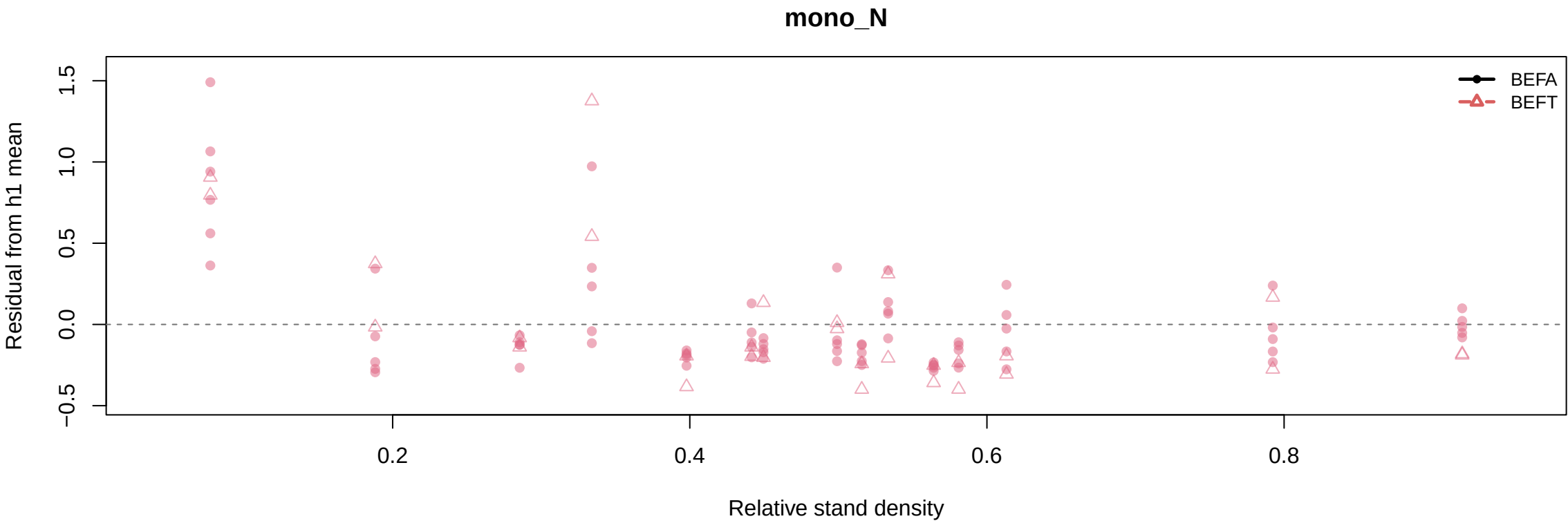
Residual from h1 mean vs rsd by h1/h2: ftp_k0_gamma
