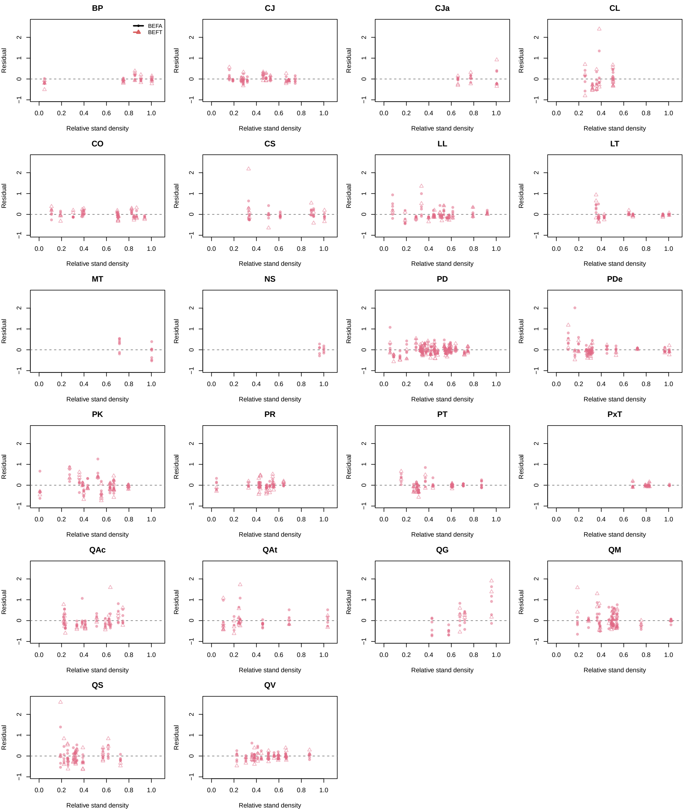
Residual vs Relative stand density by h1/h2: sp_k1_gamma
