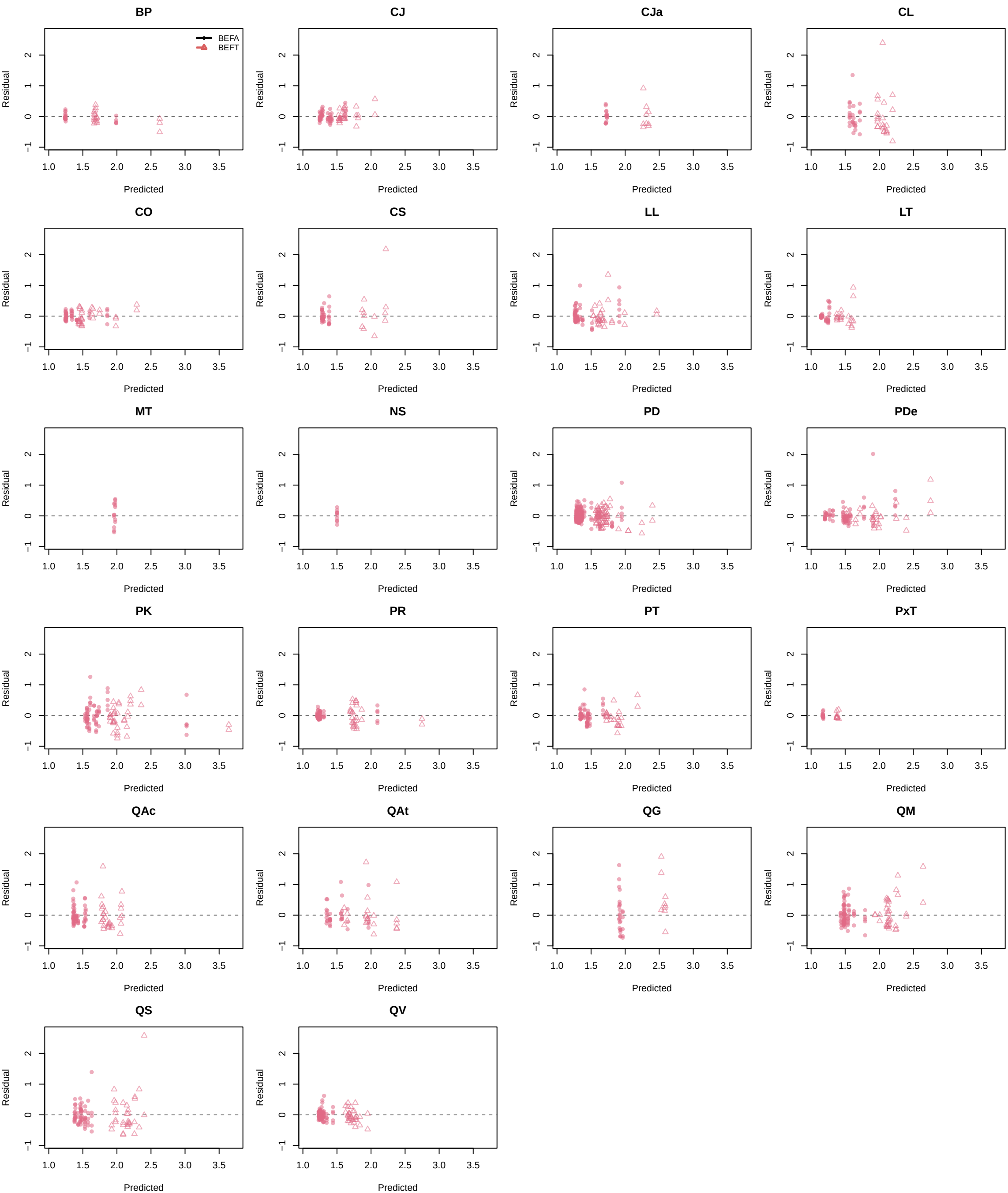
Residual vs Predicted by h1/h2: sp_k1_gamma
