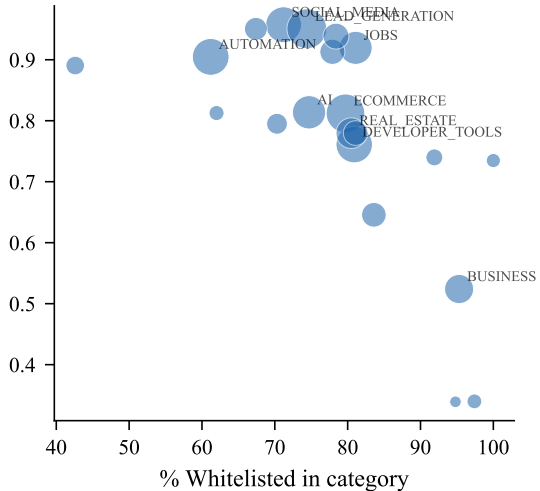
Gini coefficient
