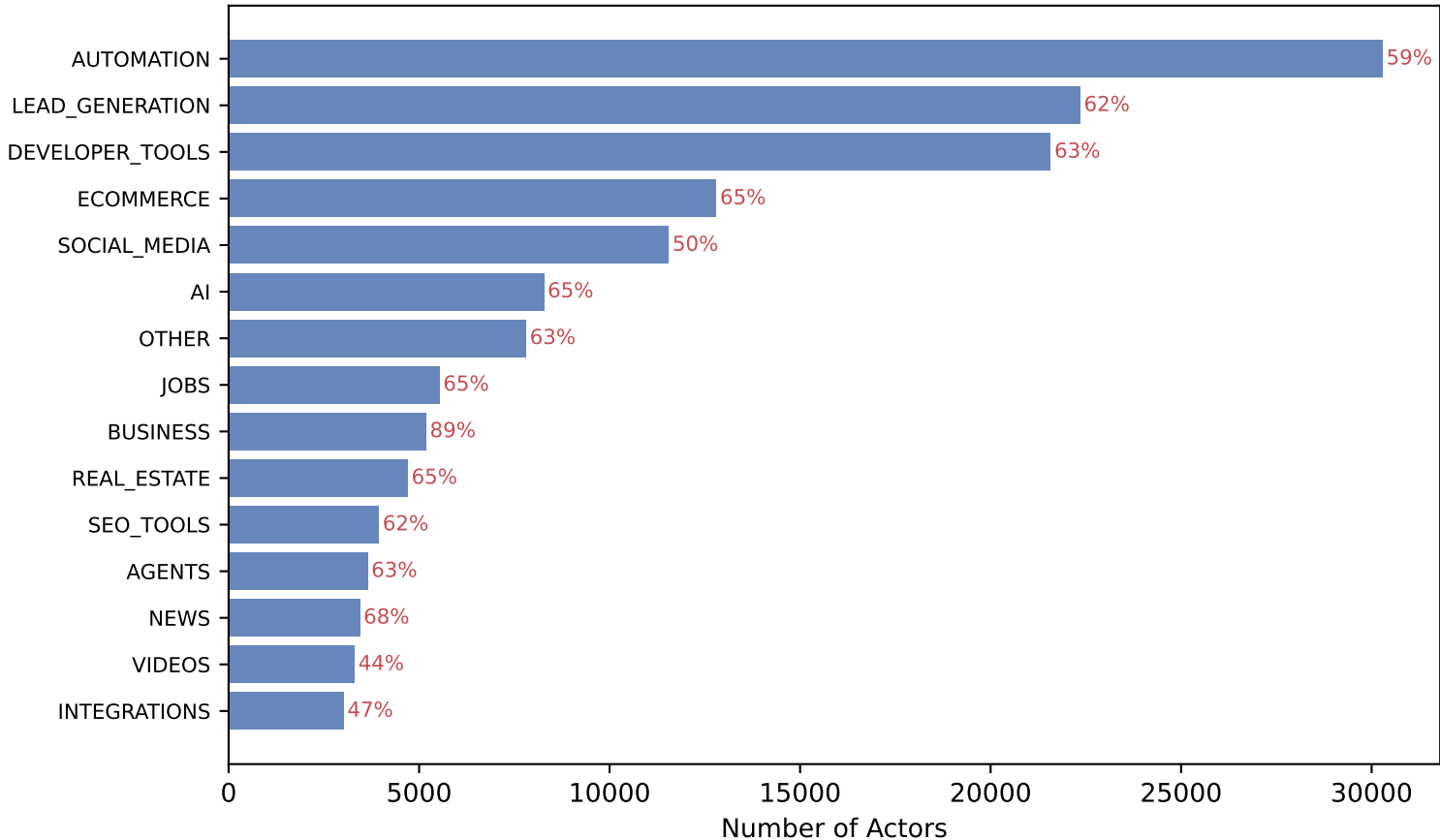
Top 15 Categories by Size (with Agentic Share %)
