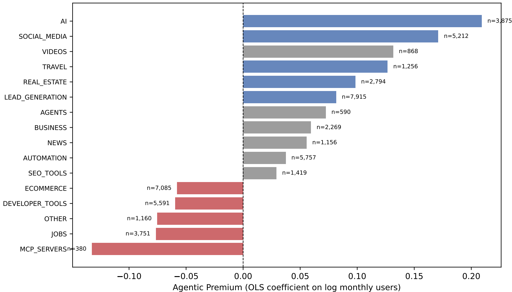
Agentic Adoption Premium by Category (blue = sig. positive, red = sig. negative, gray = n.s.)
