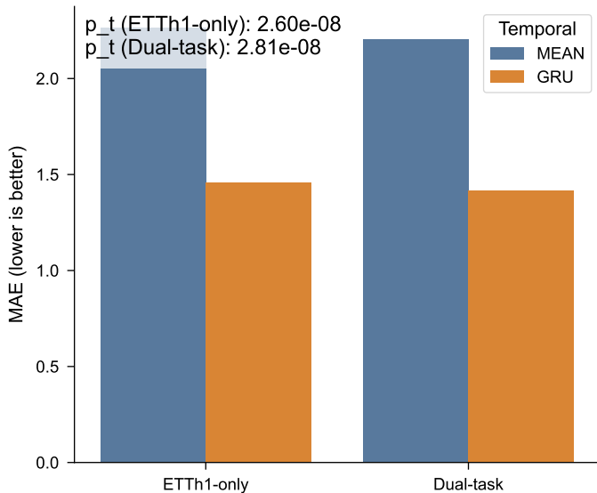
F3a. ETTh1 MAE by Temporal Control
