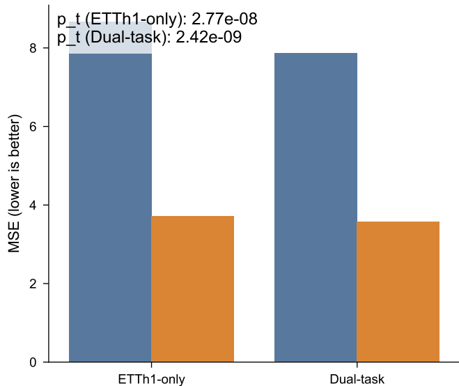
F3b. ETTh1 MSE by Temporal Control
