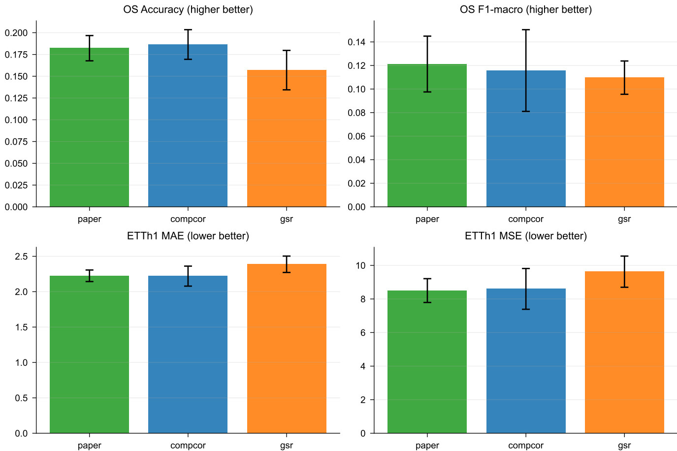
Robustness Draft Fig B: Nuisance Sensitivity (MoBSE n100, s=10)
