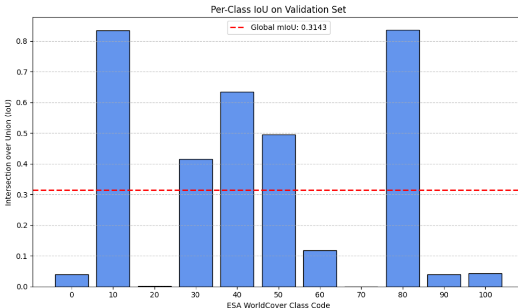
Figure 4: Per-class IoU bar chart (produced inline in the notebook). The dashed red line marks the global mIoU of 0.3143.
