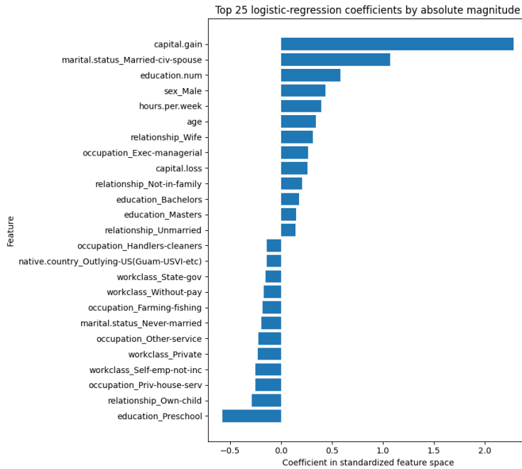
Figure 3: Logistic Regression coefficients
