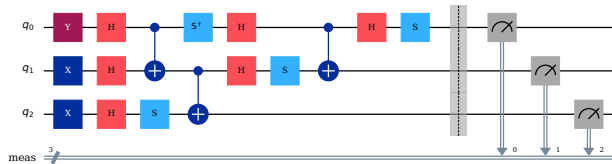
Circuit 7: Random Clifford (d~8)
