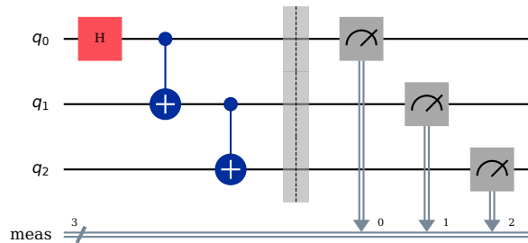
Circuit 5: GHZ (0->1->2)
