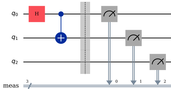
Circuit 3: Bell (0, 1)
