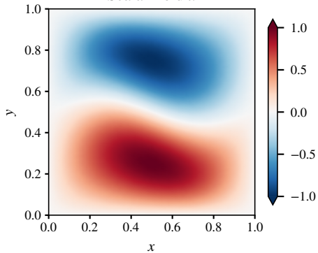
(a) Reference Scalar field u
