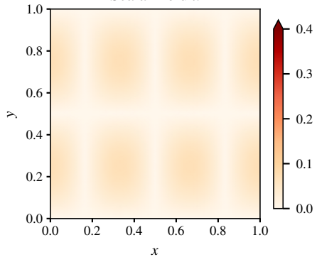
(c) Absolute error Scalar field u
