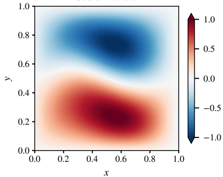
(b) Synthetic prediction Scalar field u
