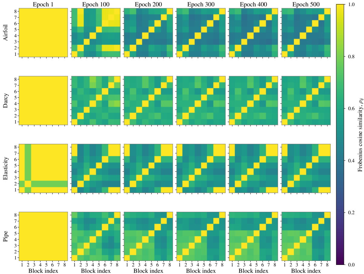
Cross-dataset evolution of matched base routing kernel WD^{-1}W^T
