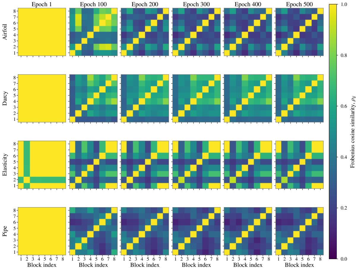
Cross-dataset evolution of matched full kernel WAD^{-1}W^T
