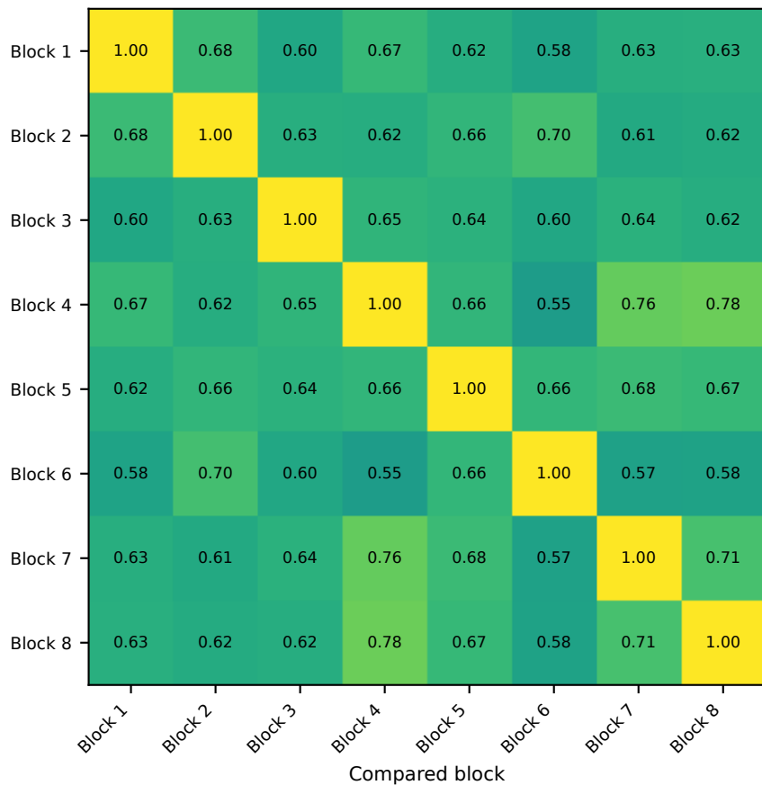
Base slice/deslice kernel
