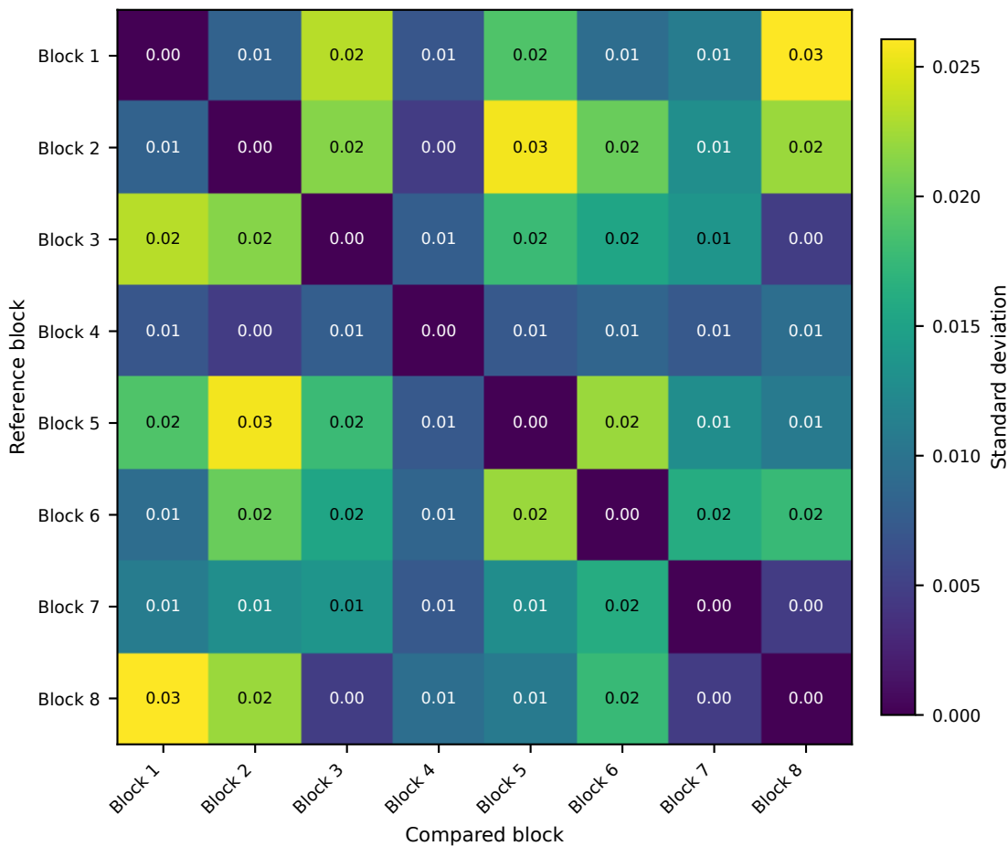
Base-kernel similarity standard deviation
