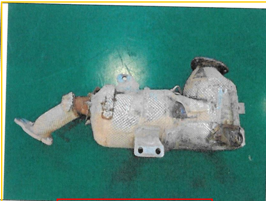
Fig.1 DOC+DPF overview
