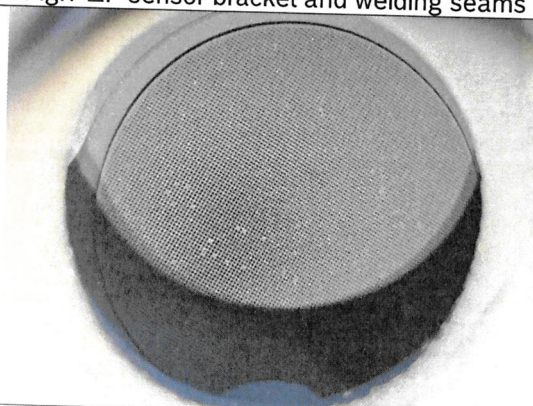
Fig.9 DOC catalyst
